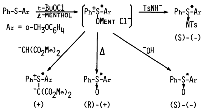
Fig. 2. Asymmetric syntheses of some optically active tricoordinate sulfur compounds.
